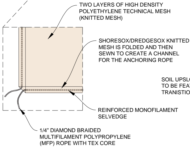
FABRIC PANEL CORNER DETAIL
